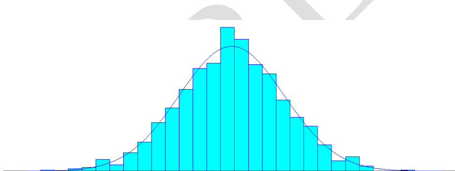
Fig. 1. The normal distribution, theoretical and sampled. Where the horizontal axis shows the value of a variable, and the vertical axis shows the relative frequency (probability) of such value. The theoretical value is in a solid line, while the sample appears as a bar in each interval. Source: Authors.
