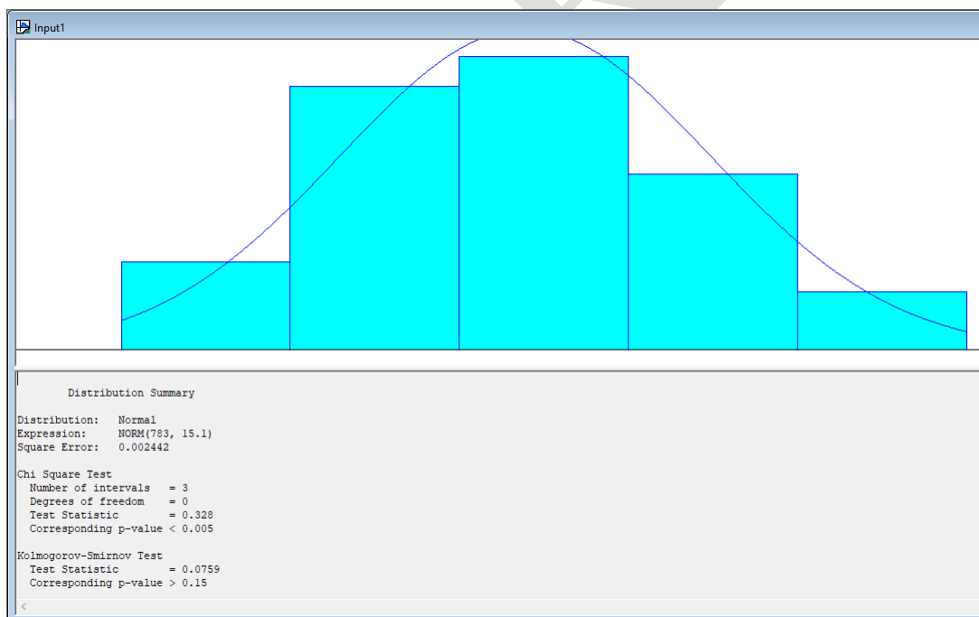
Fig. 6. Distribution of average number of fruits per plant after taking 30 simulations for 3 different hectare layouts.
