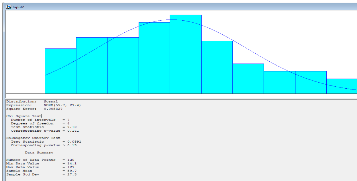
Fig. 4. Statistical analysis of the weight harvested from the sample. Source: Authors.
